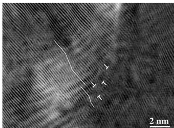
FIG. 2. A HREM image showing severe lattice distortion near a nonequilibrium GB.
