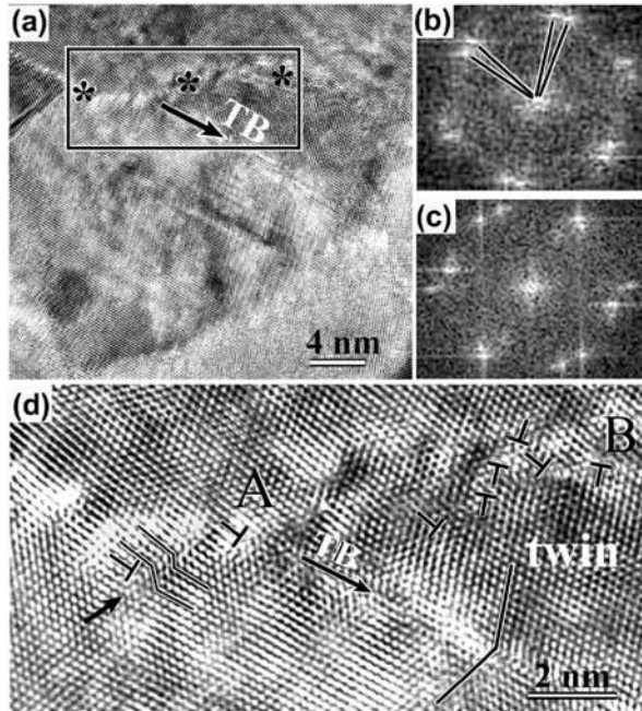
FIG. 1. (a) A HREM image showing a low angle ( \sim 3^\circ ) GB (marked with asterisks) and a twin lamellar with the twin boundary (TB) marked by an arrow. [(b) and (c)] Fourier filtered diffraction patterns of the low angle GB and twin, respectively. (d) An enlarged image of the area inside the frame in (a).
