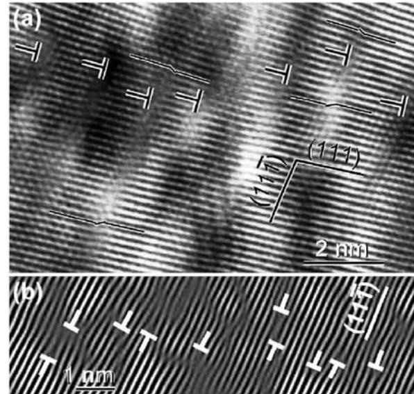
FIG. 3. HREM images showing (a) dissociation of 60^\circ dislocations into Shockley partials bounding stacking faults on a nonequilibrium GB and (b) an inverse Fourier transformation image of high density dislocations on (11\bar{1}) planes. The arrow indicates the GB direction.
