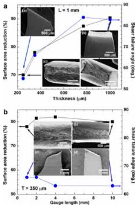
Figure 3. Thickness (a) and gauge length (b) effects on fracture surface area reduction and shear failure angle of the UFG Cu. The insets are SEM images of the fracture orientations and surfaces of the UFG Cu with L = 1 \text{ mm} and T = 250 \mu\text{m} and 1 \text{ mm} , respectively (a), and T = 350 \mu\text{m} and L = 1 and 10 \text{ mm} , respectively (b).
